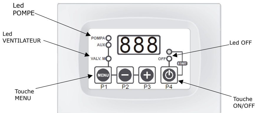
Figure 10 - Display
